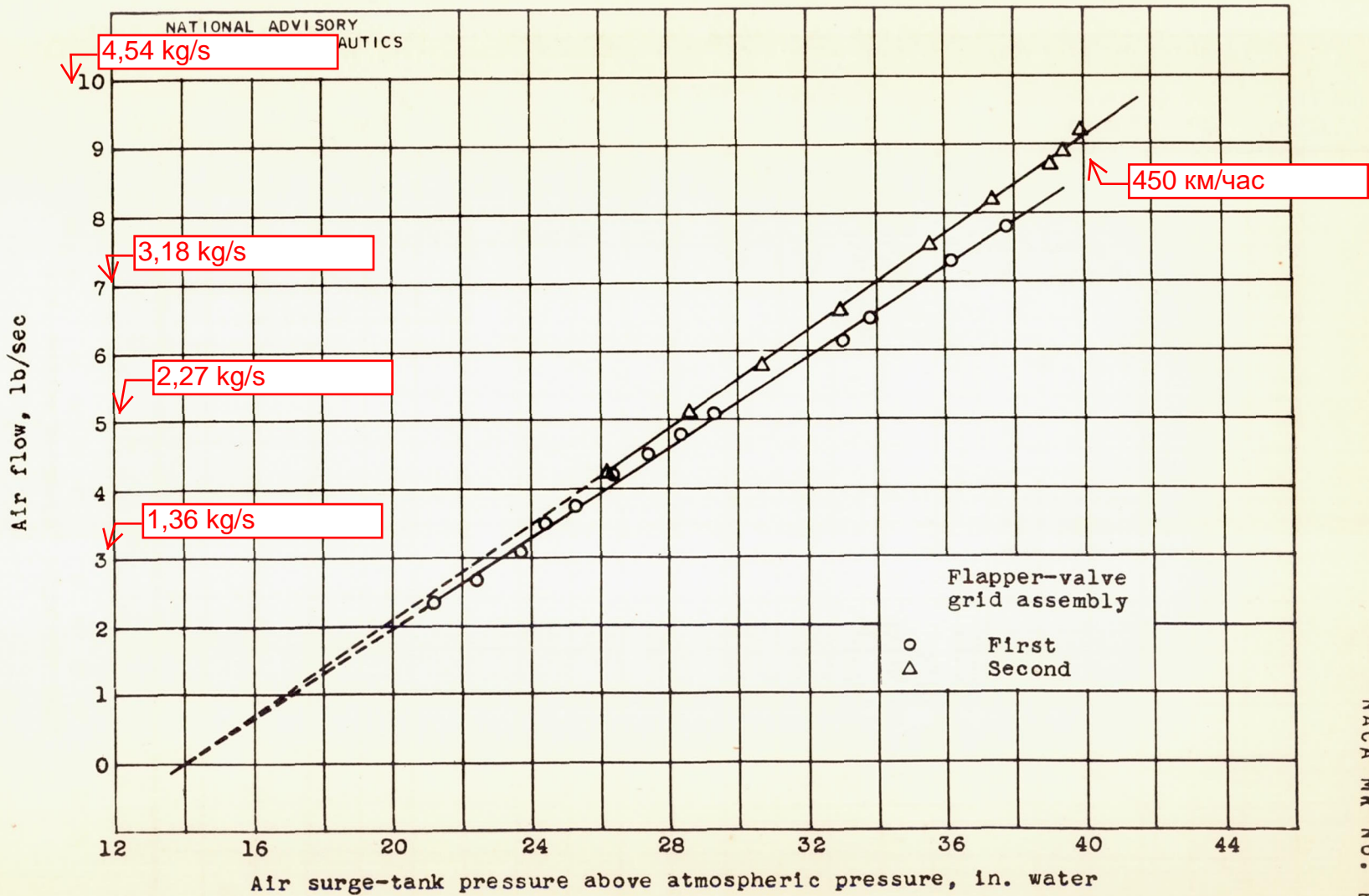
Figure 18.- Pressure-loss characteristics of the two flapper-valve grid assemblies in the performance tests.
